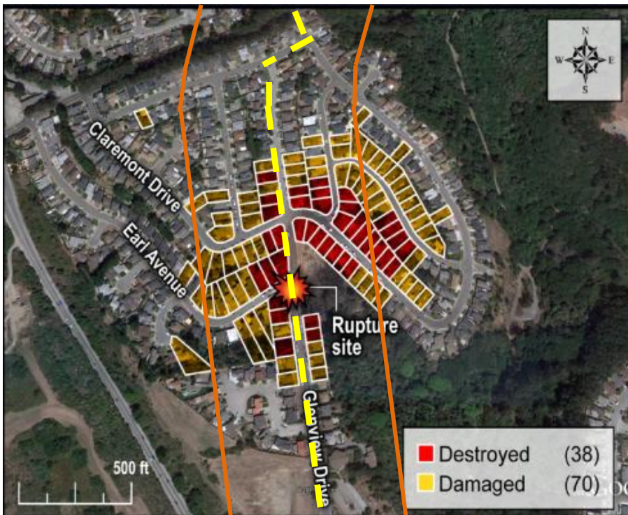
Impact Area, Natural Gas Transmission Pipeline Explosion San Bruno, CA
